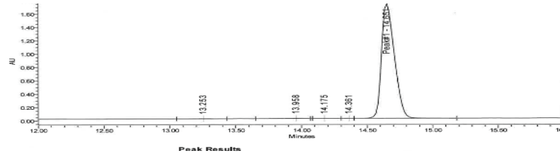
HPLC-UV Chromatogram
