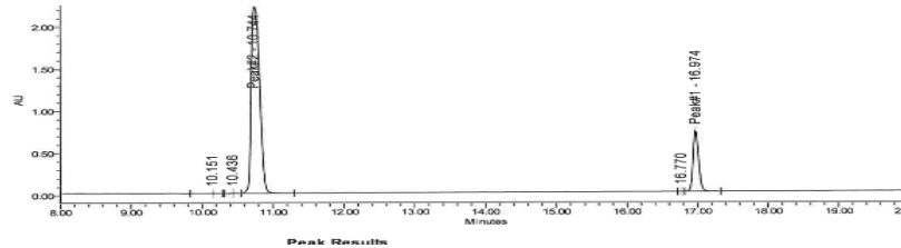
HPLC-UV Chromatogram
